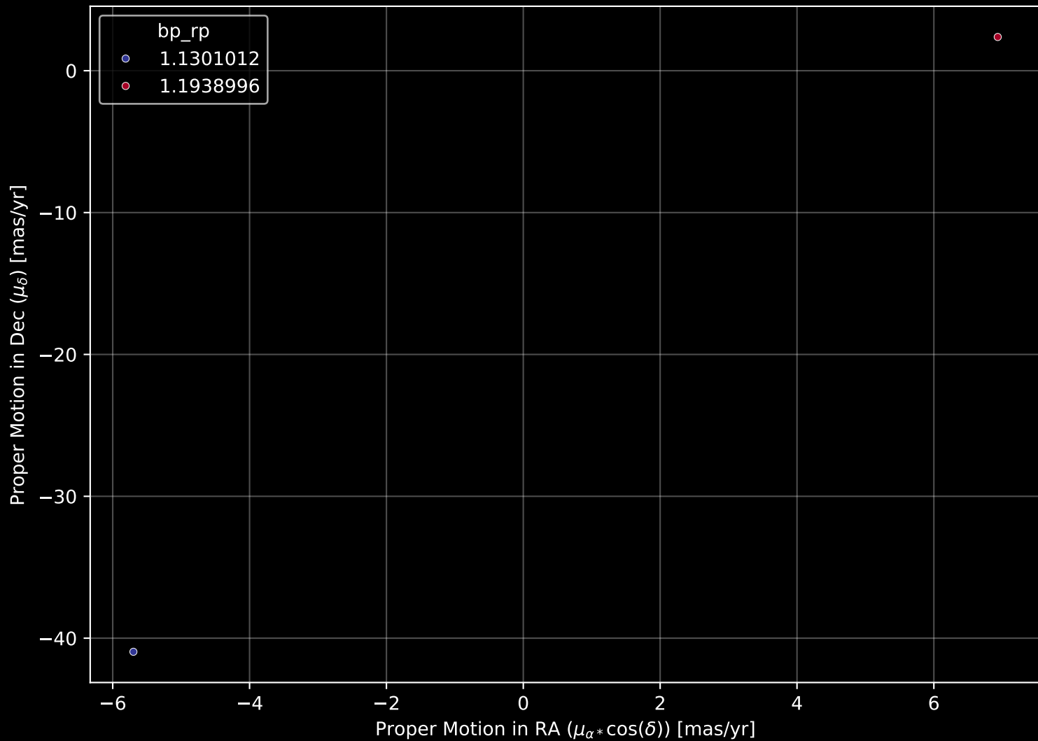
APOGEE DR17 Field: [RCB] Proper Motion Diagram (n= 2)
