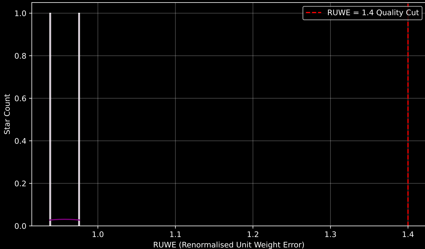
GAPOGEE DR17 Field [RCB] RUWE Distribution (n= 2)
