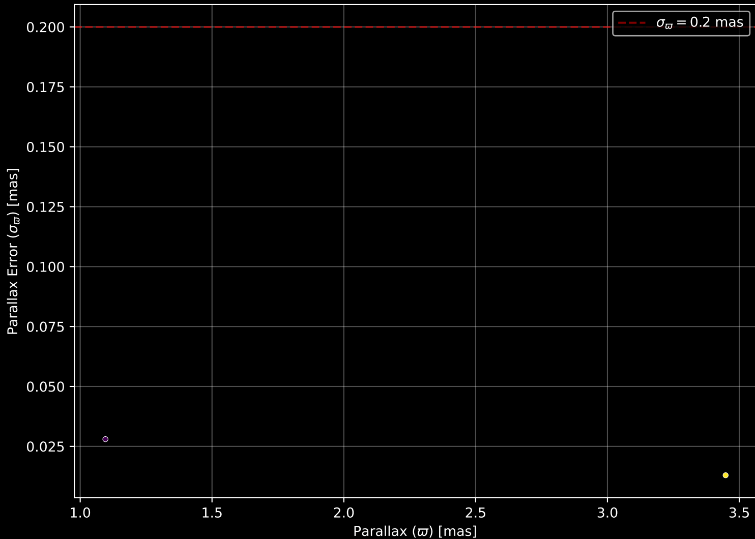
APOGEE DR17 Field: [RCB] Parallax Quality (n= 2)
