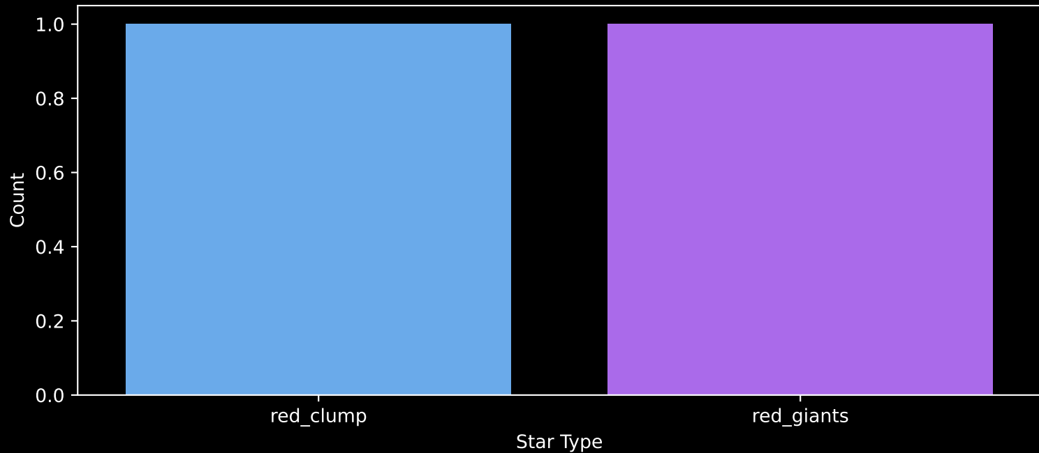
APOGEE DR17 Field: [RCB] Count plot of Star Type
